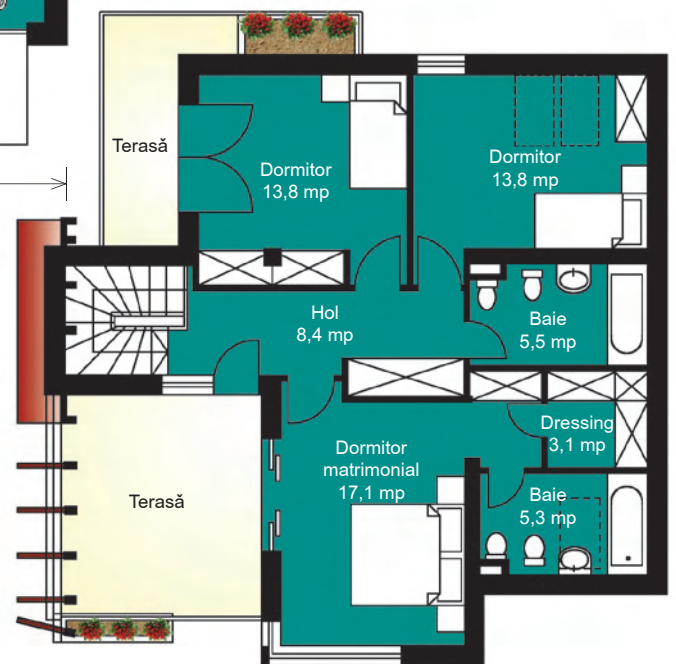
PLAN MANSARDĂ
